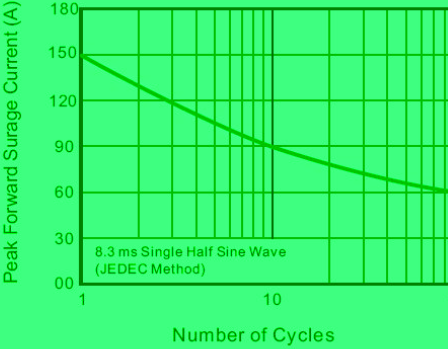
Forward Surge Current
