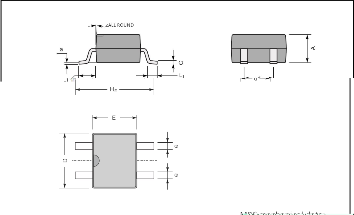
MBS mechanical data
